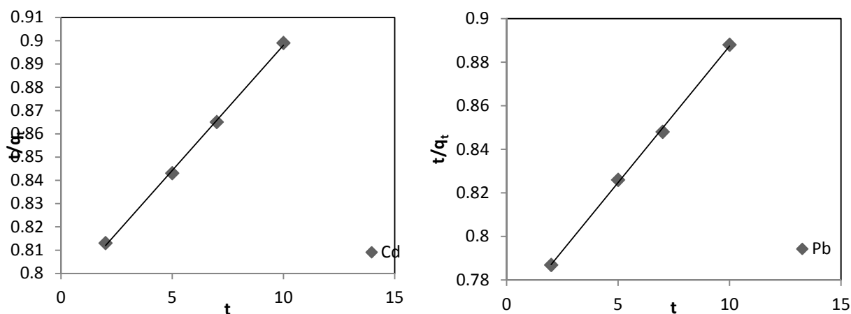
Fig. 8. Pseudo second-order kinetics for adsorption of \text{Cd}^{2+} and \text{Pb}^{2+} ions by calix[4] arene.
