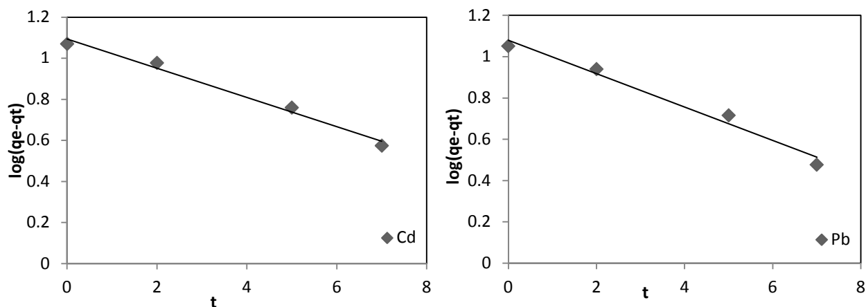
Fig. 7. Pseudo first-order kinetics for adsorption of (a) \text{Cd}^{2+} and (b) \text{Pb}^{2+} ions by calix[4] arene.
